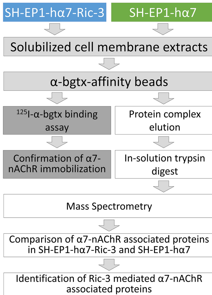
Fig 1. Experimental design. Five biological replicates of both SH-EP1-h \alpha 7 -Ric-3 cells and SH-EP1-h \alpha 7 cells were independently processed and analyzed. Triton X-100 solubilized \alpha 7 -nAChR protein complexes were isolated from SH-EP1-h \alpha 7 -Ric-3 and SH-EP1-h \alpha 7 extracts using \alpha -bgtx-affinity beads. Binding of \alpha 7 -nAChRs to affinity beads was confirmed with 125 I- \alpha -bgtx radioligand binding assays. Separately, \alpha 7 -nAChR protein complexes isolated from SH-EP1-h \alpha 7 -Ric-3 and SH-EP1-h \alpha 7 were eluted from affinity beads using 1 M carbachol. Eluted proteins were reduced and alkylated before being digested with trypsin in-solution. Digested peptides from each of the five samples prepared from SH-EP1-h \alpha 7 -Ric-3 and SH-EP1-h \alpha 7 cells were analyzed with a Q Exactive mass spectrometer, spectra identified using the Mascot algorithm and results analyzed using ProteoIQ. Identified \alpha 7 -nAChR associated proteins from SH-EP1-h \alpha 7 -Ric-3 and SH-EP1-h \alpha 7 cells were compared. Associations only identified with Ric-3 co-expression in SH-EP1-h \alpha 7 -Ric-3 cells were determined to be Ric-3-mediated changes in the \alpha 7 -nAChR interactome.
