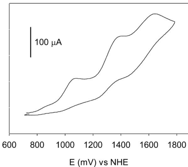
Figure 4. Cyclic voltammogram of [\text{Ru}(\text{bpy})_2\text{PMe}_3(5\text{HT})]^{+2} recorded in acetonitrile at 100 mV/s on Pt wire electrode in \text{CH}_3\text{CN} containing 100 mM \text{TBAPF}_6 as supporting electrolyte.
