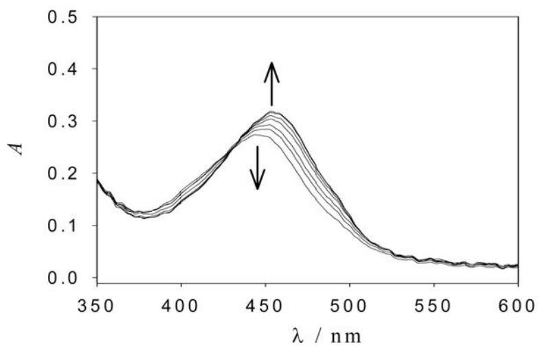
Figure 2. Subset of UV-vis spectra of [\text{Ru}(\text{bpy})_2(\text{PMe}_3)(5\text{HT})]^{2+} acquired in aqueous solution at pH = 7 while irradiating with a 405 nm laser diode. The arrows indicate photolysis progress.
