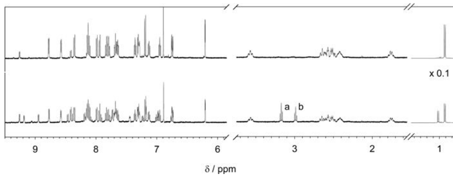
Figure 1. 1 H NMR spectra of a 5 mg/mL solution of [Ru(bpy) 2 (PMe 3 )(5HT)]Cl in D 2 O before irradiation (upper trace); and after 60 s irradiation with 525 nm green LED inside the NMR tube (lower trace). Note that after irradiation the triplets a and b appear, characteristics of free serotonin.
