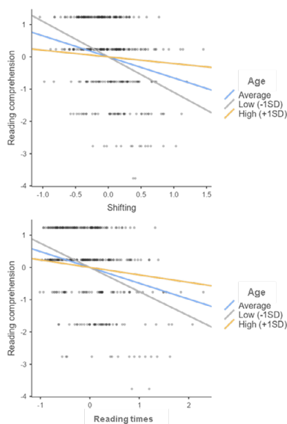
Figure 4 Slope analysis of moderation effects.
