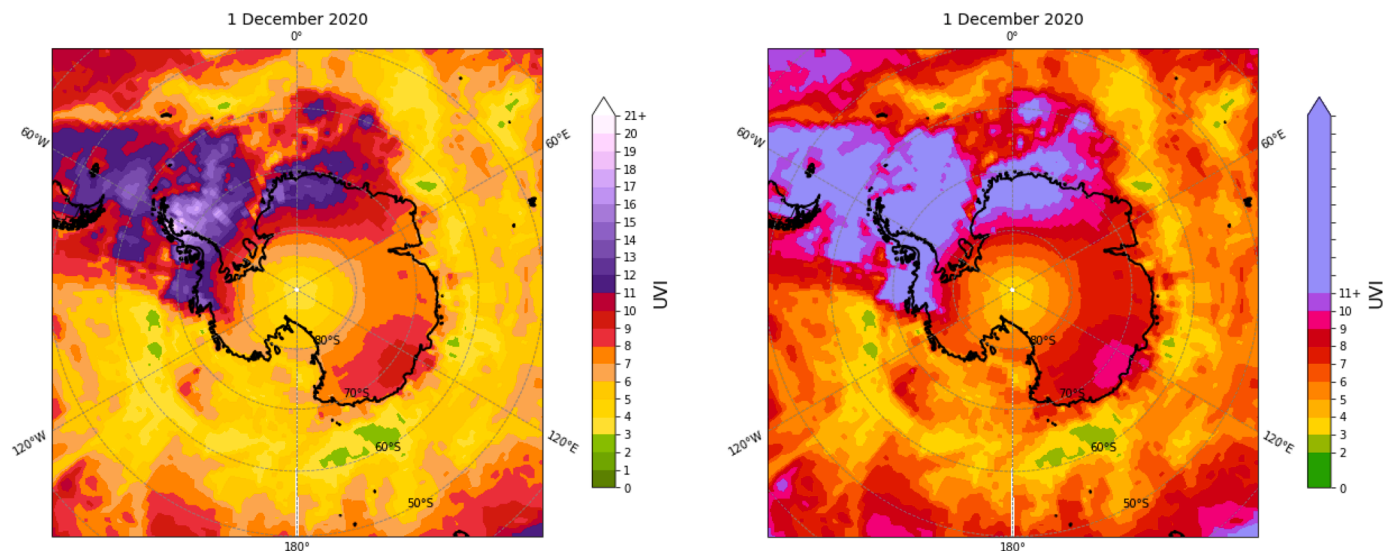
Fig. D3. Application of the proposed UCP_{UVI} (left) and comparison with the WHO [55] UCP_{UVI} (right) to an overpass event of the Antarctic ozone hole through continental areas of southern South America and its surroundings during day 01 December 2020. Noon all-sky UVI data provided by CERES ( https://ceres.larc.nasa.gov/index.php ).
