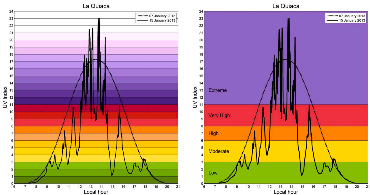
Fig. 1. Application of the proposed new UCP UVI (left) and of the standard color palette by risk ranges [55] (right) to UVI measurements recorded every 1 min during 07 January 2013 (under clear-sky conditions) and 15 January 2013 (with scattered clouds) at La Quiaca station (22.11°S, 65.57°W, 3459 m a.s.l.) of the Argentine UV Monitoring Network.
