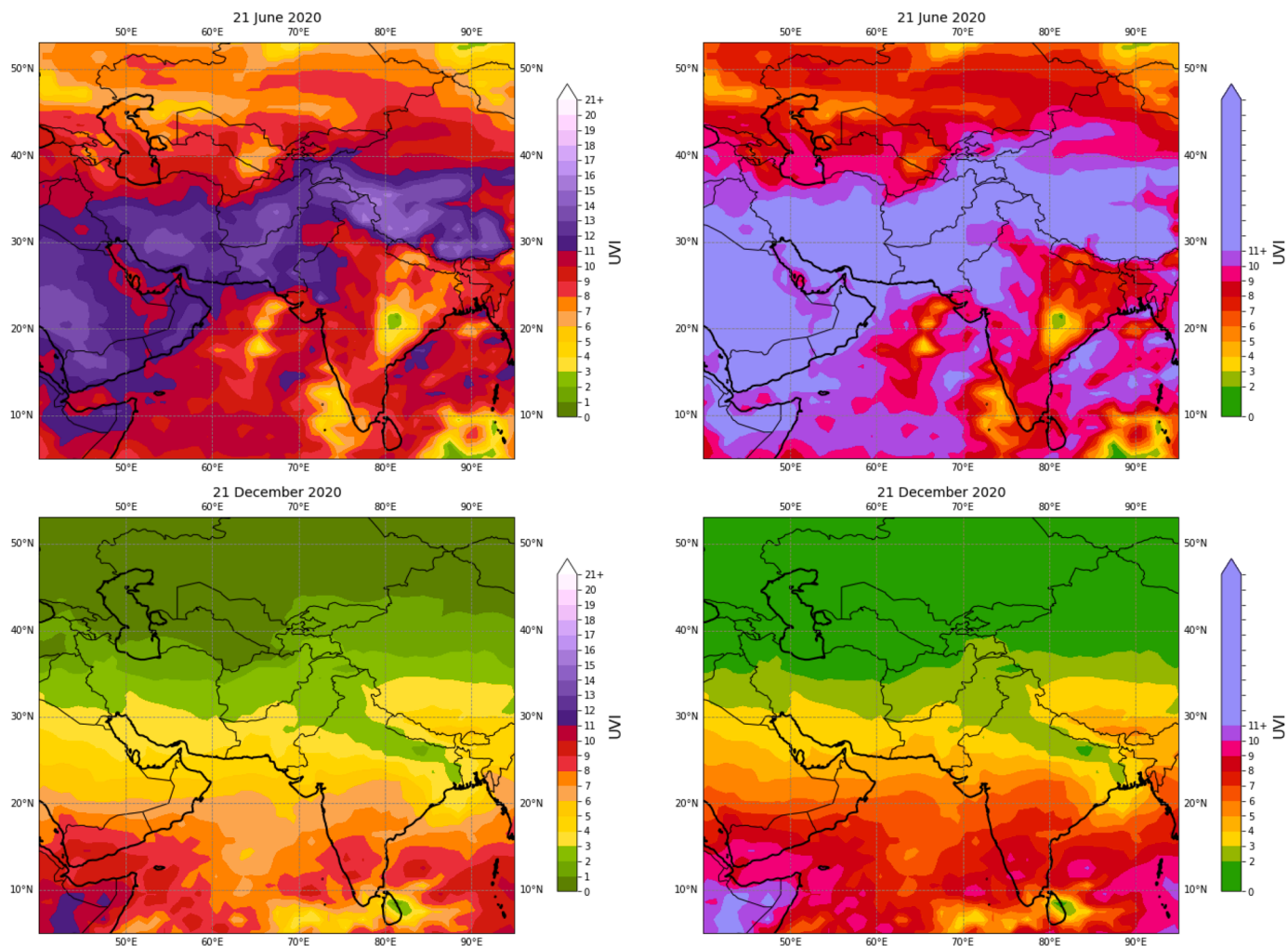
Fig. D2. Application of the proposed UCP_{UVI} (left) and comparison with the WHO [55] UCP_{UVI} (right) to a zoom on the maps of Fig. 3 spanning the highlands territory of the Tibet and its surroundings for 21 June 2020 (top) and 21 December 2020 (bottom).
