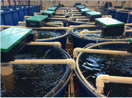
Figure1: An example of recirculating aquaculture systems (RAS) located at the Virginia Tech Department of Food Science and Technology (Blacksburg, VA, USA). (Image taken from Wikipedia; https://en.wikipedia.org/wiki/Recirculating_aquaculture_system ).
