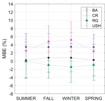
Figure 5. Seasonality of the MBE for each site. Dots indicate OMI – Dobson comparison while triangles indicate daily average OMI – SAOZ comparison. BA: Buenos Aires; CR: Comodoro Rivadavia; RG: Río Gallegos; USH: Ushuaia.
